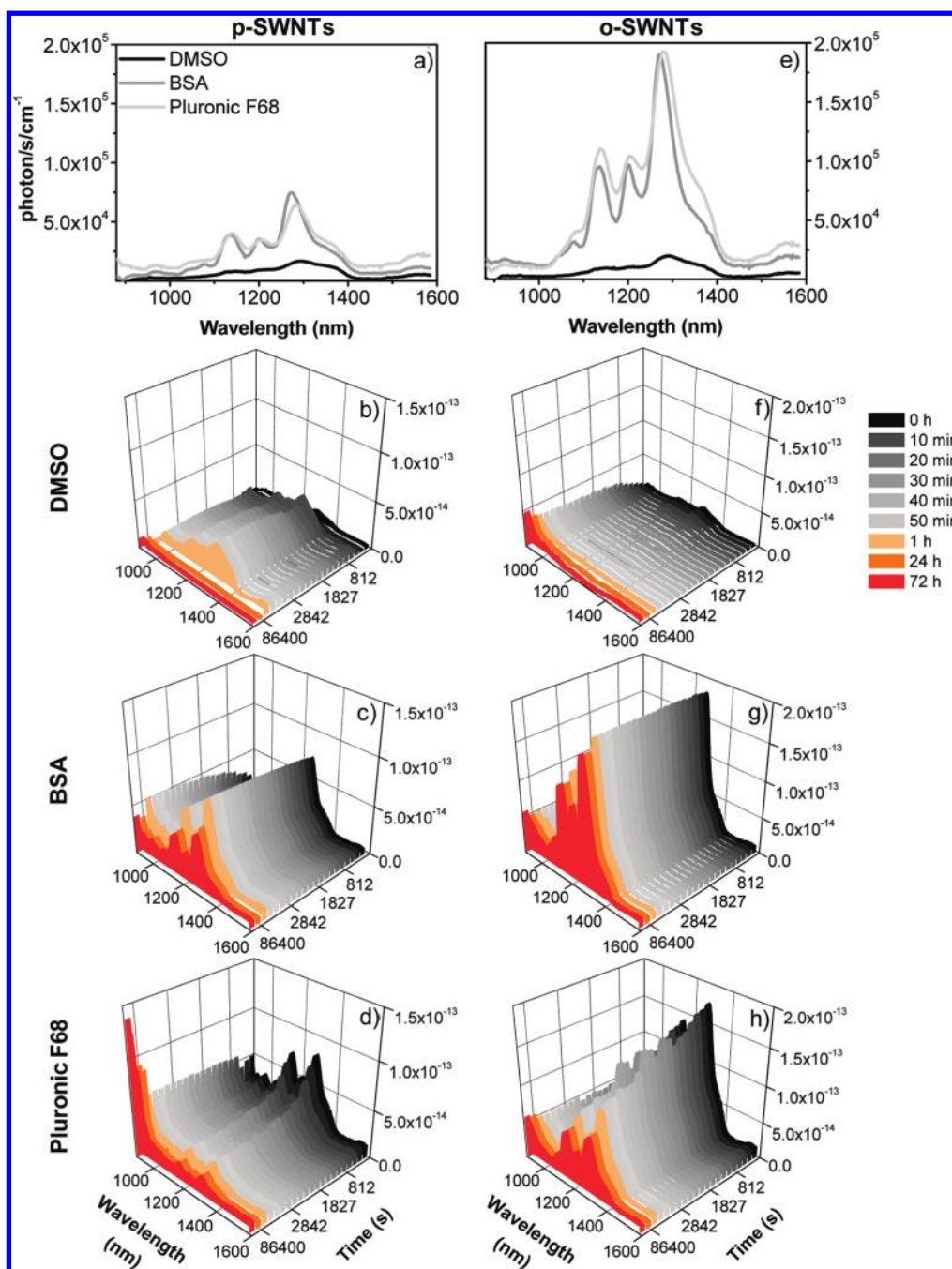
Figure 1. NIR-PL spectra ( \lambda_{exc} = 683 nm) of (a–d) p- and (e–h) o-SWNTs dispersed in supplemented RPMI 1640 cell media ( [SWNTs]_i = 120 \mu\text{g/mL} ) with or without the addition of a dispersing agent (BSA or Pluronic F68). Graphs (b–d; f–h) show the changes of NIR-PL of (b, f) DMSO-, (c, g) BSA-, and (d, h) Pluronic F68-stabilized dispersions over 1 h (black to light orange curves), after 24 h (orange curves) and after 72 h (red curves).
