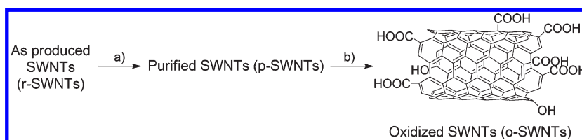
Scheme 1. Purification and oxidation of as-produced HiPCO SWNTs (r-SWNTs): 31 (a) \text{HNO}_3 2.6 M, 100 °C, 48 h; (b) \text{H}_2\text{SO}_4 \cdot \text{H}_2\text{O}_2 (4:1), 35 °C, 1 h.
