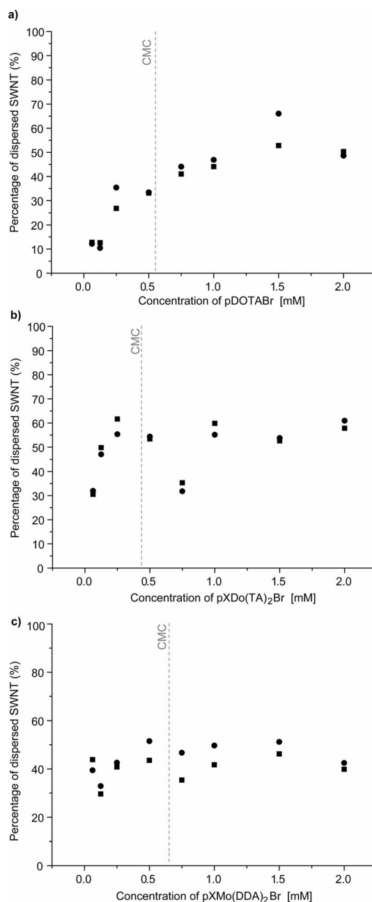
Figure 3. Percentage of SWNTs dispersed with a) pDOTABr, b) pXDo(TA) 2 Br and c) pXMo(DDA) 2 Br (real absorbance/theoretical absorbance determined at 377 nm taking advantage of the calibration curve constructed by Di Crescenzo et al. [23] with \epsilon_{377 \text{ nm}} = 106.0 \text{ mL/mg cm} ). Circles and squares refer to different experiments performed under the same experimental conditions.
